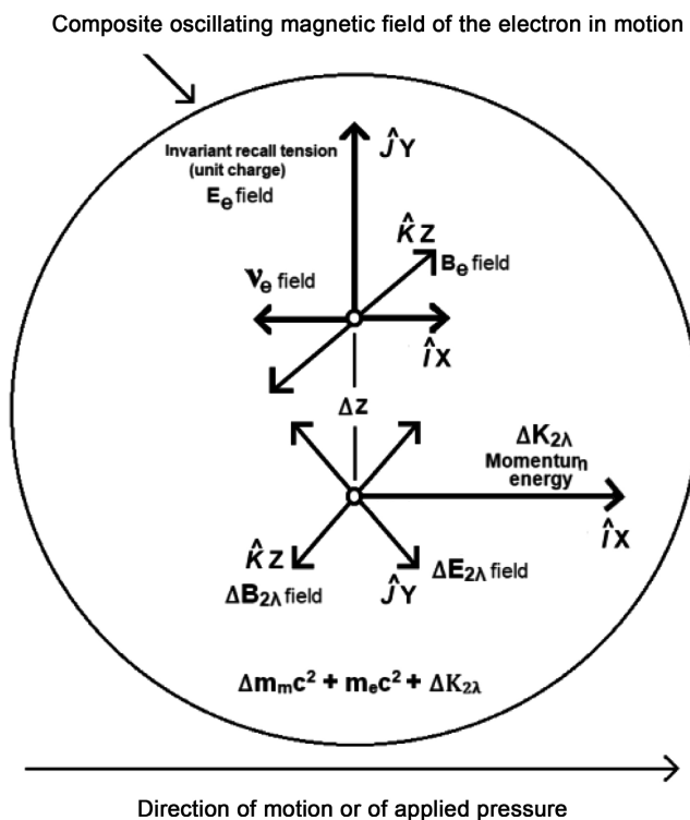
Figure 9. The trispacial vector complex of the relativistic mass of the electron in motion and of its momentum energy—level 2 trispacial vector complex.
