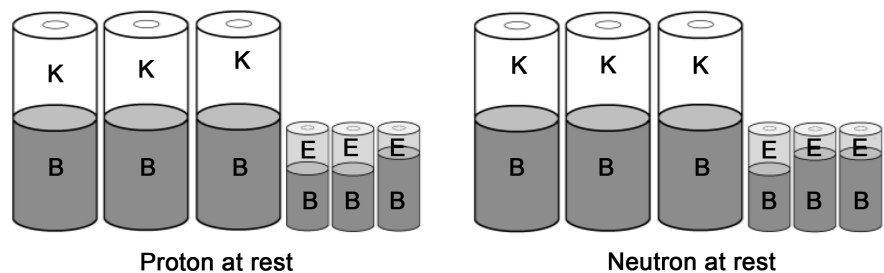
Figure 15. The energy which is part of the proton and neutron rest masses.
