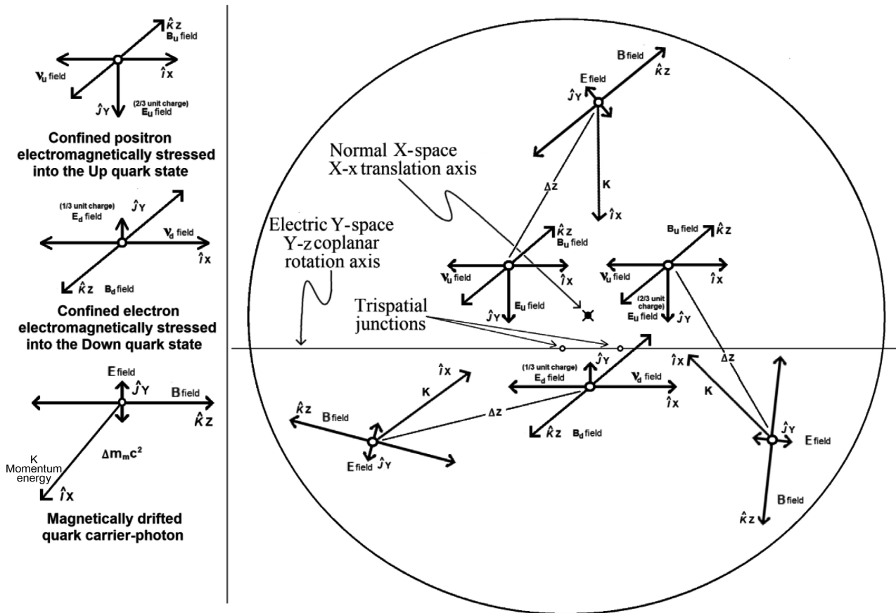
Figure 13. The proton at rest—level 2 trispatial vector complex.
