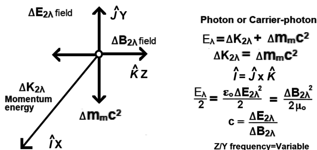
Figure 8. The trispacial vector complex of a photon or carrier-photon—level 0 trispacial vector complex.
