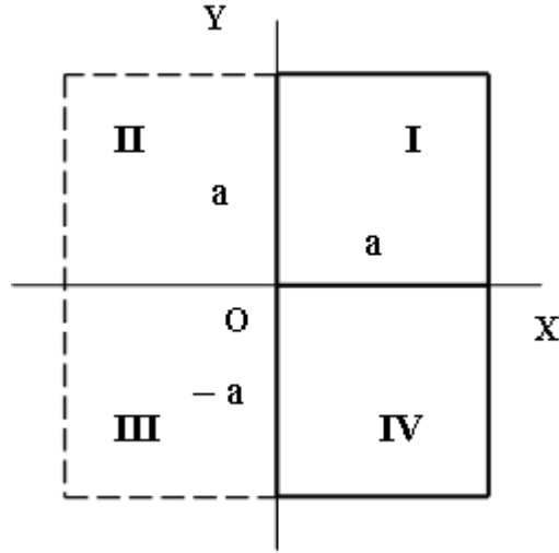
Figure 1. The position of the material geometrical figure “square with identical sides a meter ” in the quarters I and IV of the coordinate system XOY .
