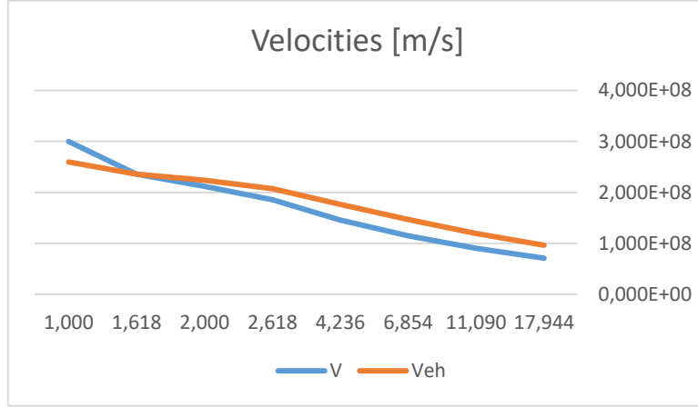
Figure 1. Velocities near to the black hole (At abscise are the products of the radius r_b = GM / c^2 )
