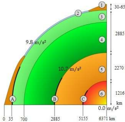
Figure 5. Schematic view of the interior of Earth. 1. continental crust - 2. oceanic crust - 3. upper mantle - 4. lower mantle - 5. outer core - 6. inner core - A: Mohorovičić discontinuity - B: Gutenberg discontinuity - C: Lehmann discontinuity. The expected gravitation field strengths are shown as well.
