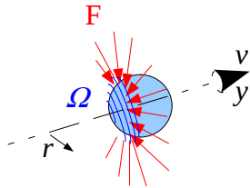
Fig. 2.4 : a particle's gyrotation field and therefore its compression is heterogeneous due to its velocity.
