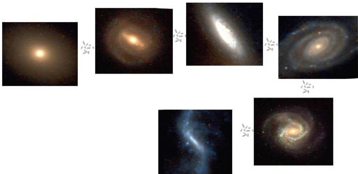
Fig.4.1: Evolutionary classification of galaxies. From spherical galaxy to an elliptic galaxy, then a disc galaxy and a spiral galaxy. After a reorientation of the bulge's angular momentum, a bar galaxy with a circularly outside-spreading turbulent zone is created, which a apocalyptic disturbance of the stars and planetary systems of the whole galaxy.
