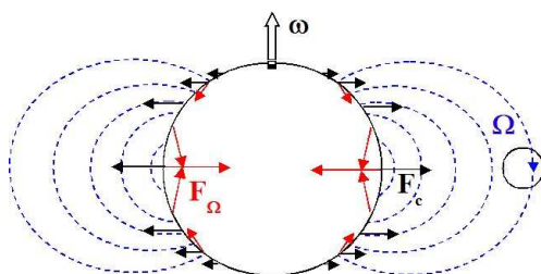
Figure 1.b. A rotating body also provides an external gyrotation \Omega that has an inverse orientation of the body's rotation.
