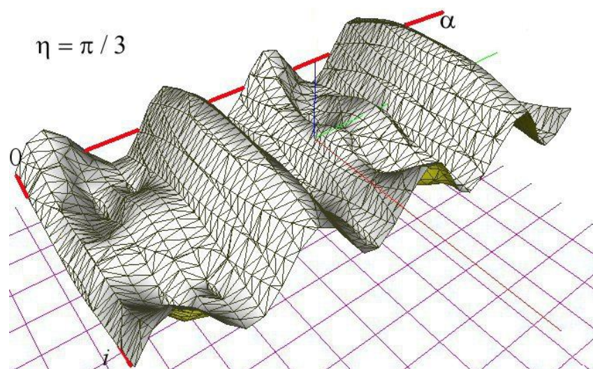
Fig. 2.5: Indicative values of the tilt change \dot{\theta} at \eta = \pi/3 .
