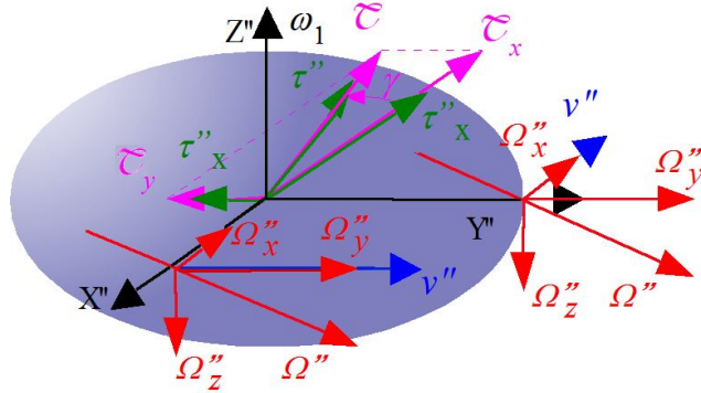
Fig. 3.4 : we consider the asteroid under the influence of the gyrotation \Omega'' . The asteroid is rigid, and the only motion-related acceleration is a''_z .
