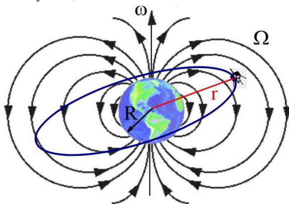
Fig. 1.1 : A spinning sphere with radius R and rotation velocity \omega is generating a rotary gravitation field (or “gyrotation” field) \Omega at a distance r from the sphere's centre.
