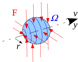
Fig. 2.2 : a particle is compressed due to its velocity.
