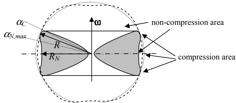
fig.3.7 : exploded rotary black hole
